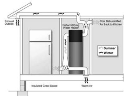
Figure 4. Air flow to and from the heat-pump water heater in
